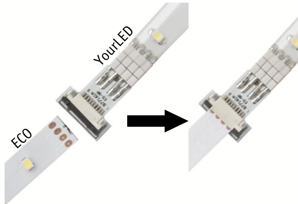
YourLED Eco Clip-to-YourLED Connector plastic white RRP €5.95 702.81
